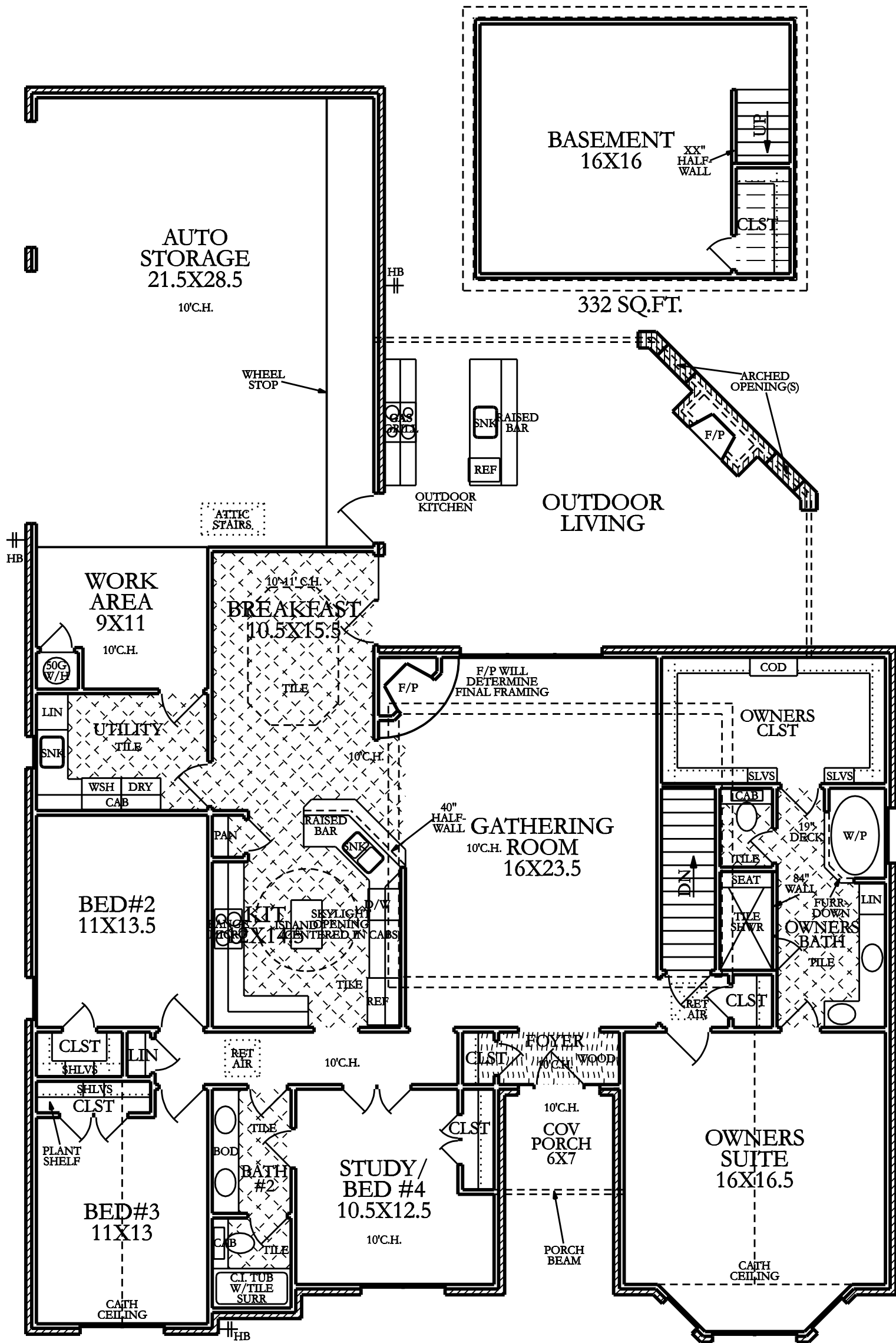
FIRST FLOOR 2289 SQ.FT.
